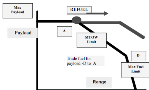
Figure 2. AAR perpetuates fuel reserves and extends range (courtesy of Nangia).
