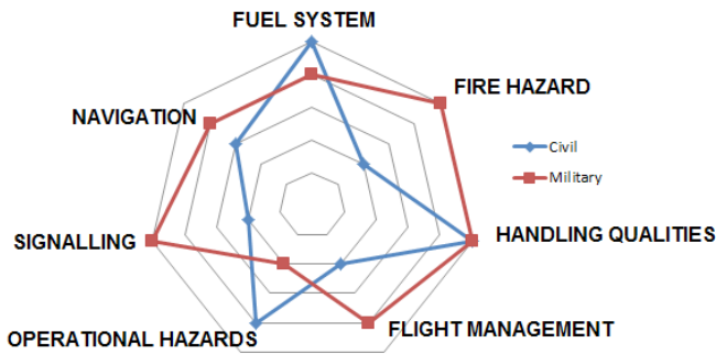
Figure 2. Contemporary capability for automatic and autonomous AAR.
