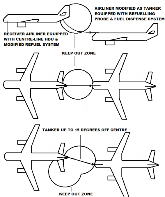
Figure 10. Viable and certifiable AAR configuration.
